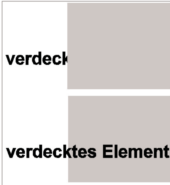
SequenceEditor
